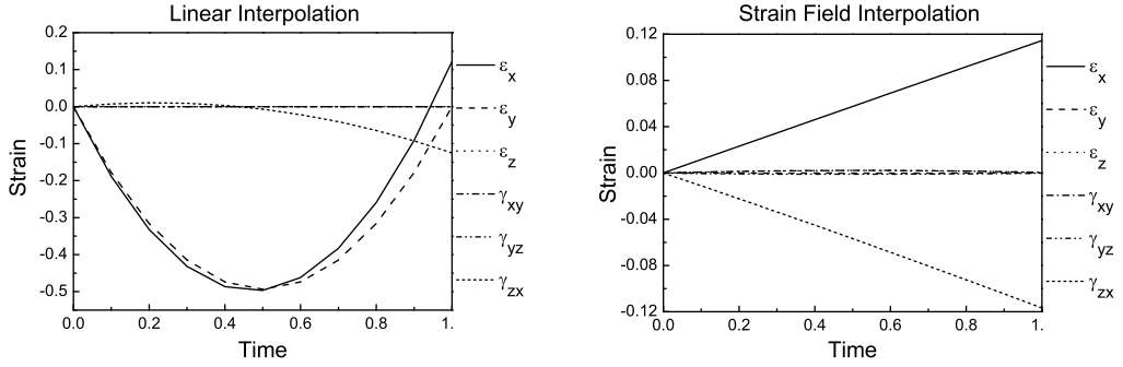
Figure 3: Strain-Time Curve
