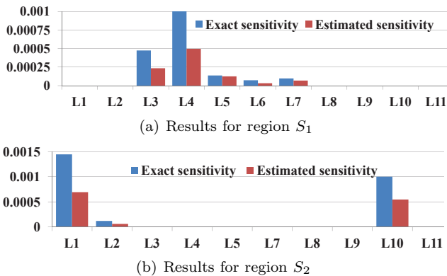
Fig. 12. The estimated modification sensitivity for each feature compared with that obtained using direct FE analysis, for the quantity defined over regions S_1 and S_2 .
