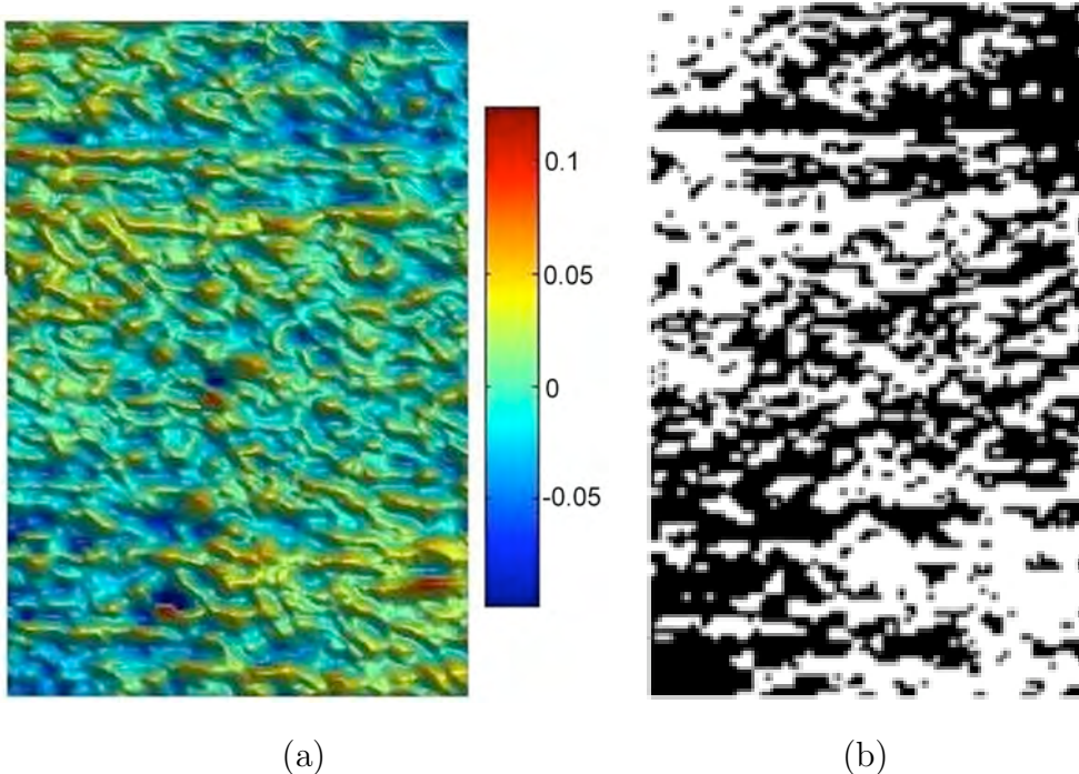
Fig. 2. Extracted noise for N1 sample given Assumption A1 (specimen rotated 90^\circ relative to Fig. 1 before scanning), else as per Figure 1.
