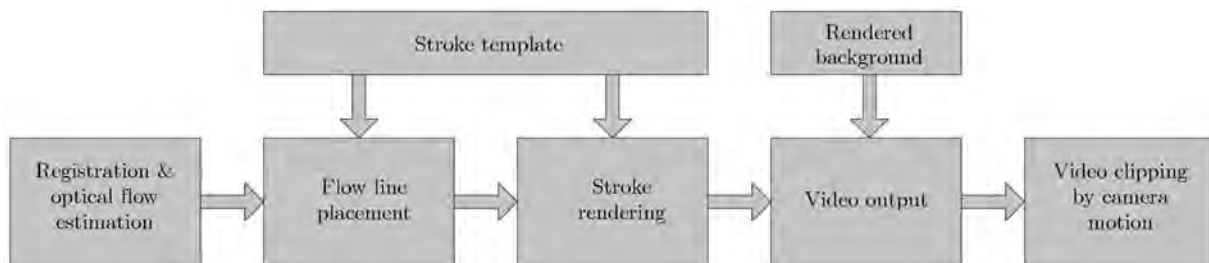
Figure 1 Processing pipeline.
