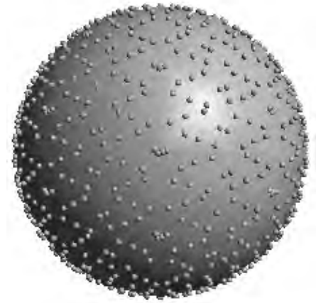
Figure 7: Niederreiter’s low discrepancy sequence of points.
