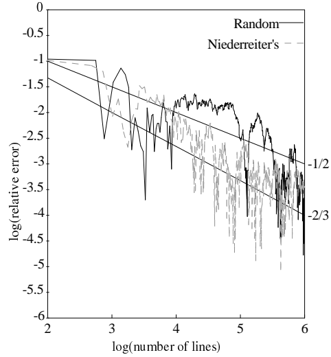
Figure 24: Errors for the 'gate', with the chord model.
