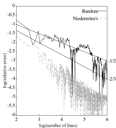
Figure 9: Errors for the sphere, with the tangent model.
