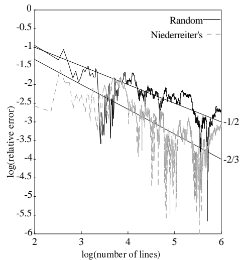
Figure 11: Errors for the object L\pm cylinder in Figure 12, with the tangent model.
