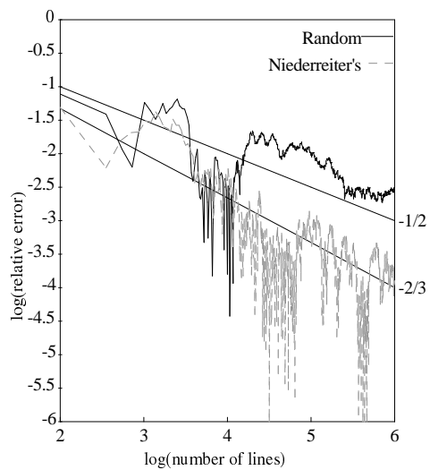
Figure 15: Errors for the sphere, with the chord model.
