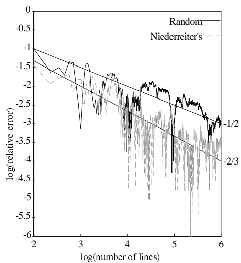
Figure 17: Errors for the L_{\pm} cylinder in Figure 12, with the chord model.
